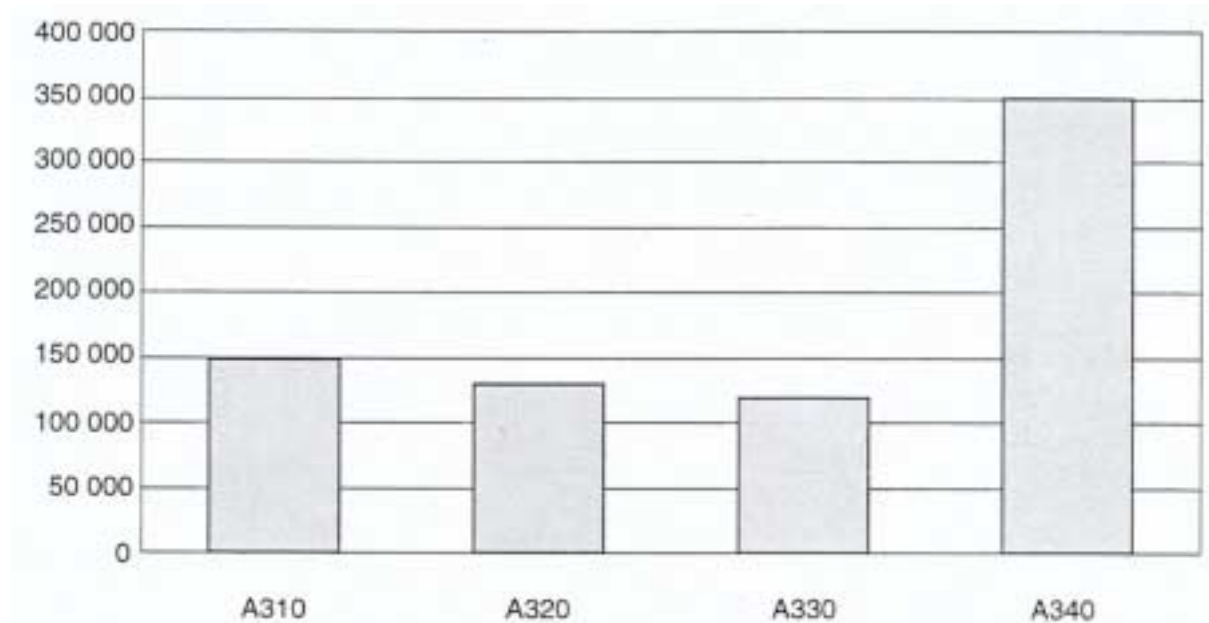
Figure 31. Potential fuel economy/year ($) 10 aircraft fleet (10 hours/day)
