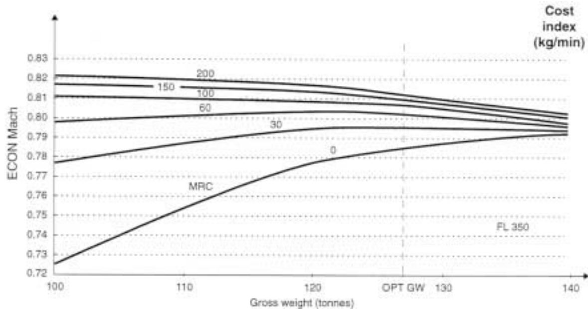
Figure 27. ECON cruise Mach = f(CI)
