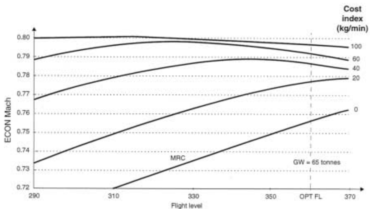
Figure 23. ECON cruise Mach = f(CI)
