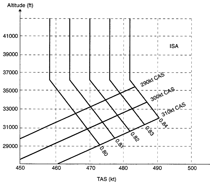
Figure 18. CAS/TAS/MACH profiles
