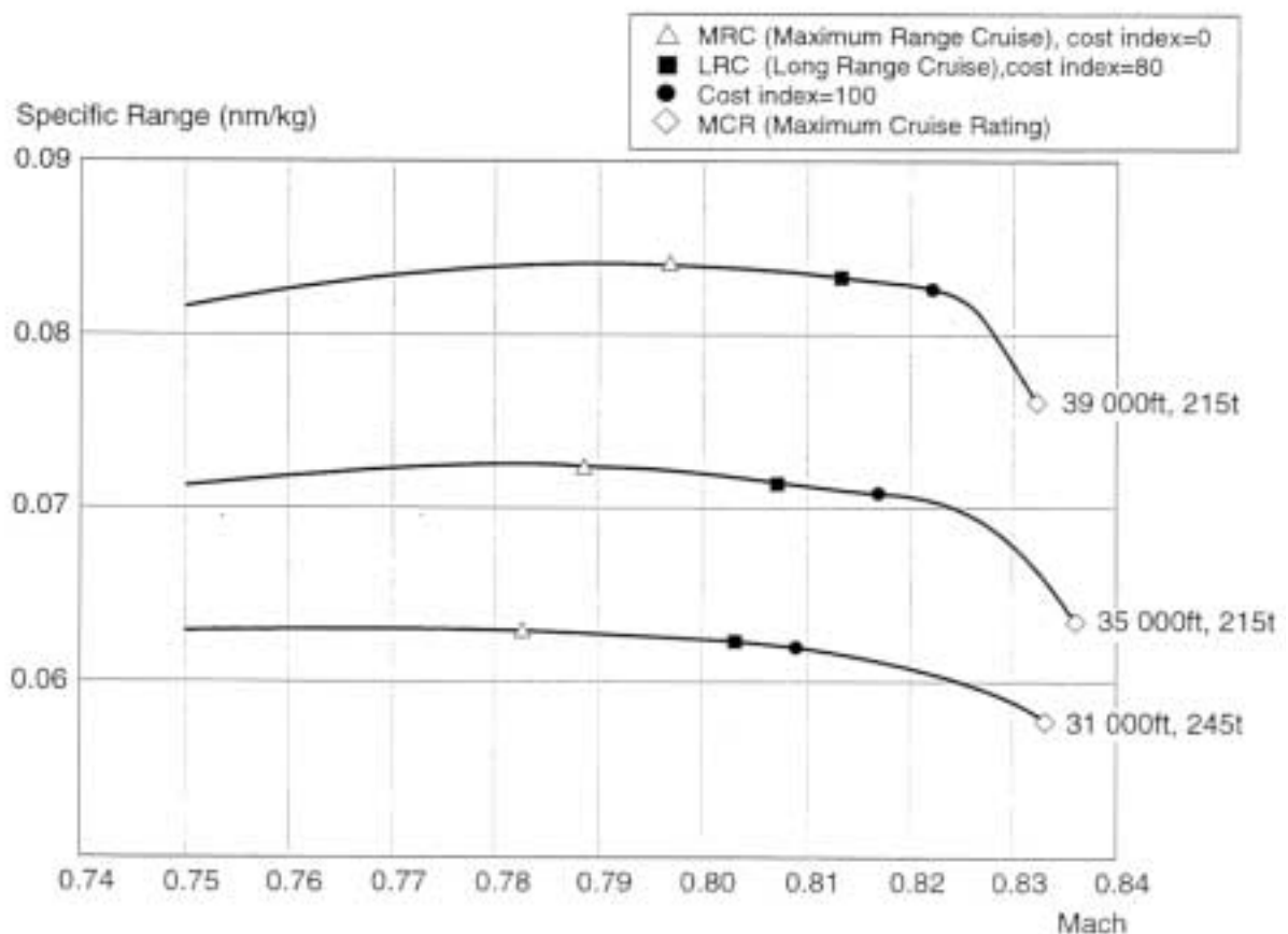
Figure 40. A340-300/CFM56-5C2, ISA
