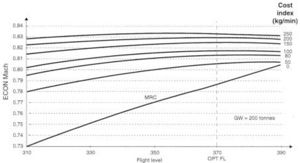
Figure 25. ECON cruise Mach = f(CI)
