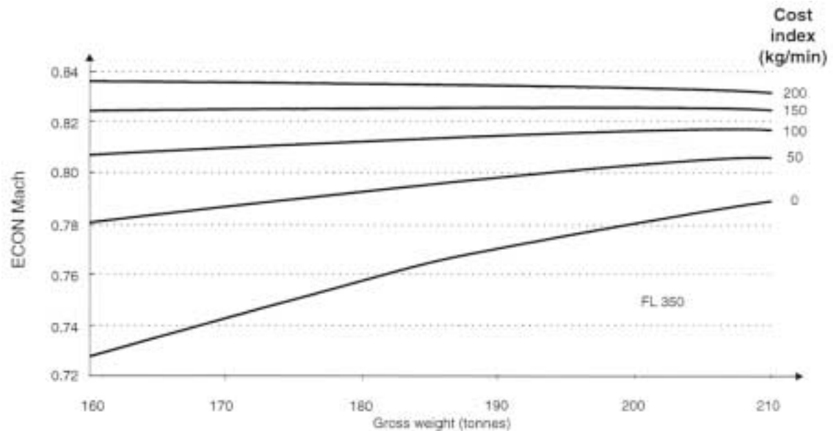
Figure 29. ECON cruise Mach = f(CI)
