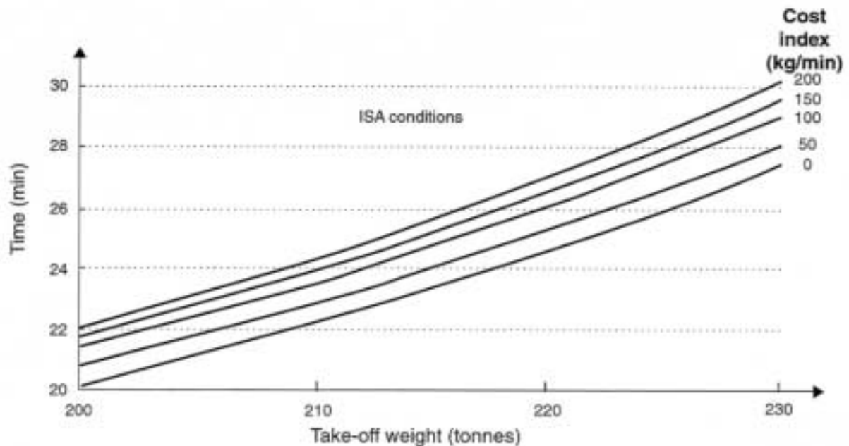
Figure 13. Time to climb to FL 350 versus CI A340-311/CFM56-5C2
